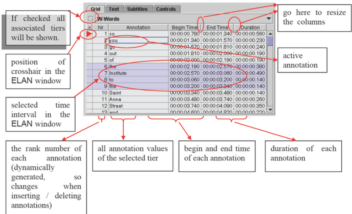
Figure 1.113. Structure of the grid viewer
