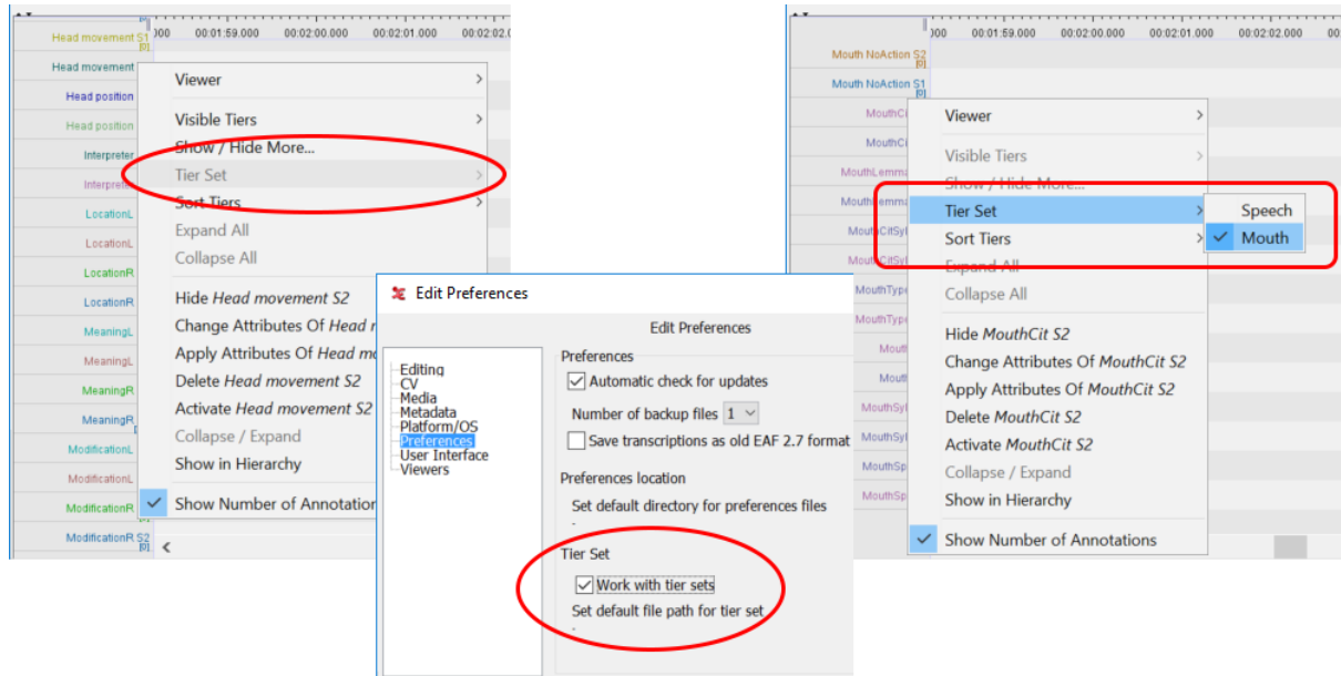
Figure 1.103. The Tier Set context menu item before and after enabling tier sets in the preferences.
