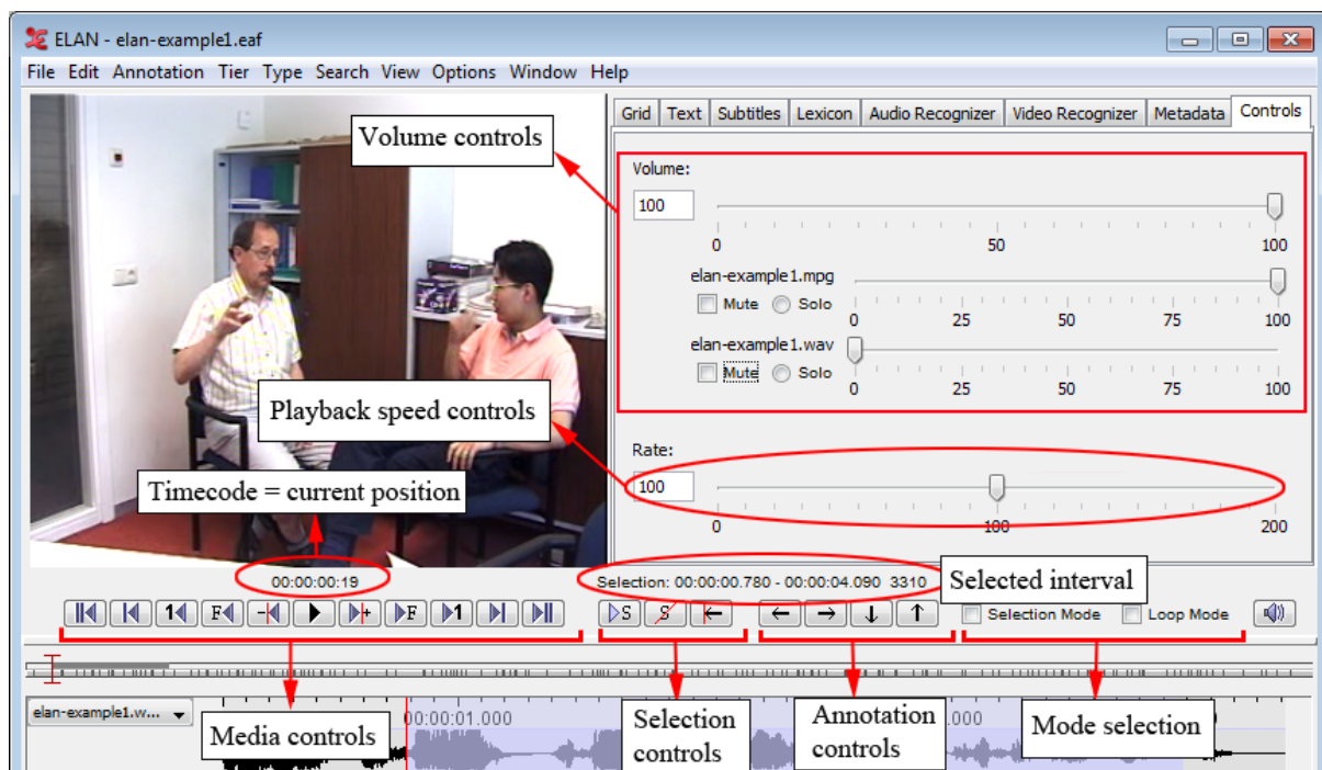
Figure 1.93. The media player options
