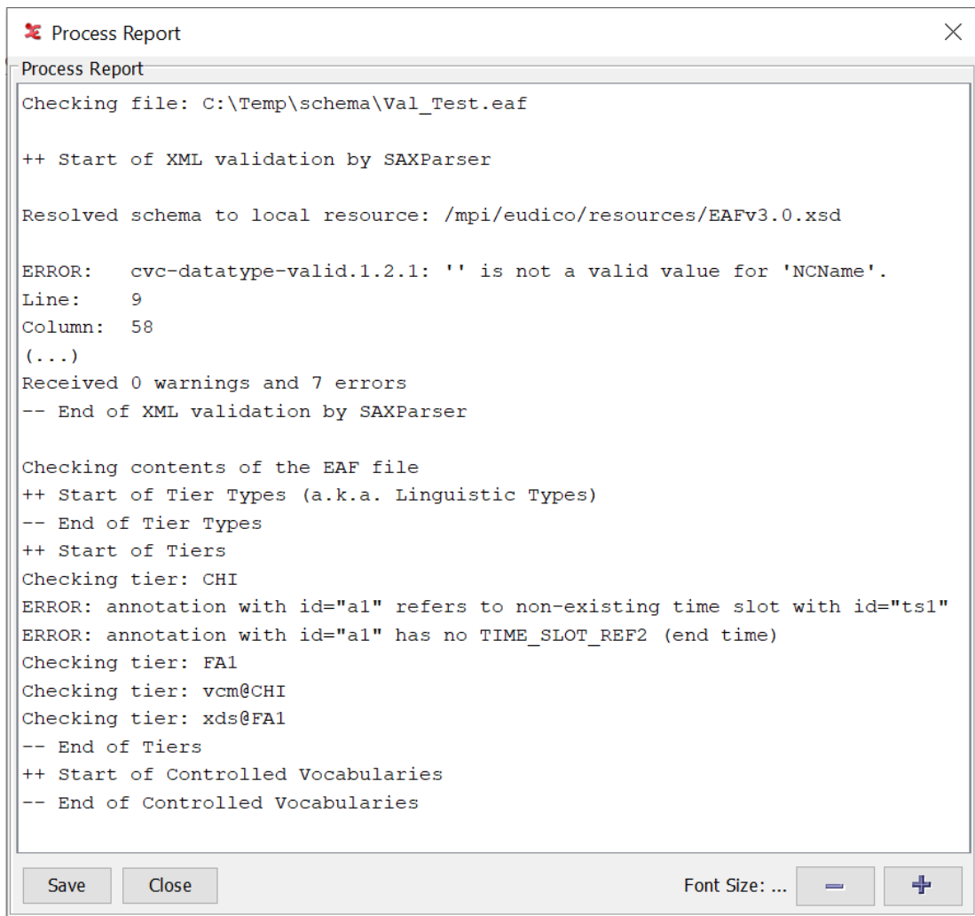
Figure 1.15. Validation report window
