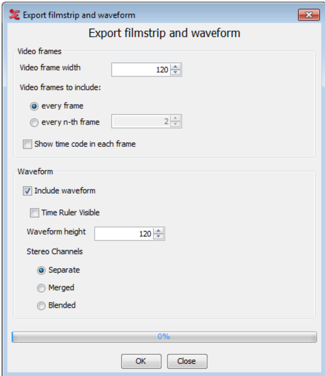
Figure 1.49. Exporting to a filmstrip image
