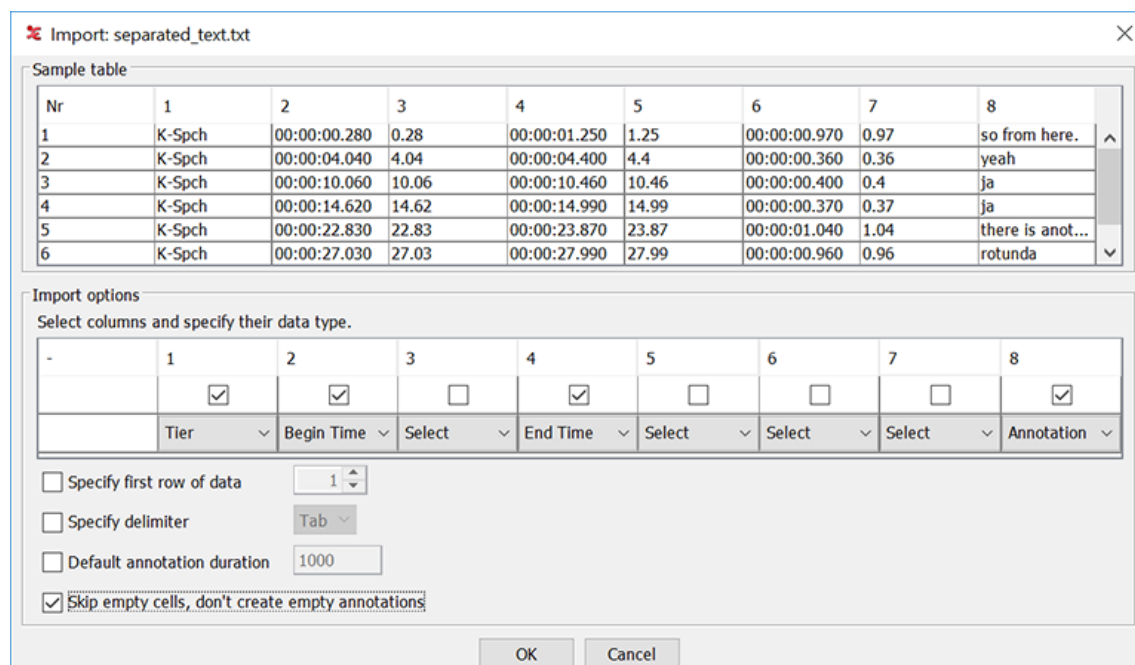
Figure 1.66. Import CSV / Tab-delimited Text
