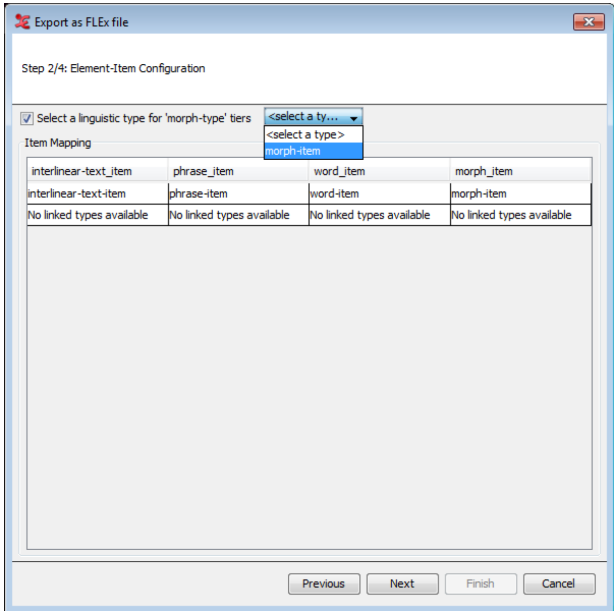
Figure 1.157. Export as FLEx file step 2
