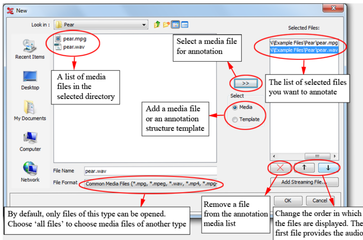
Figure 1.2. The New Transcription dialog window: media
