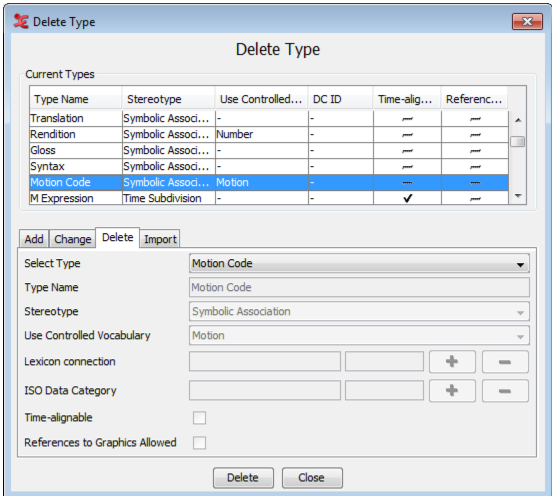
Figure 2.8. Delete a tier type
