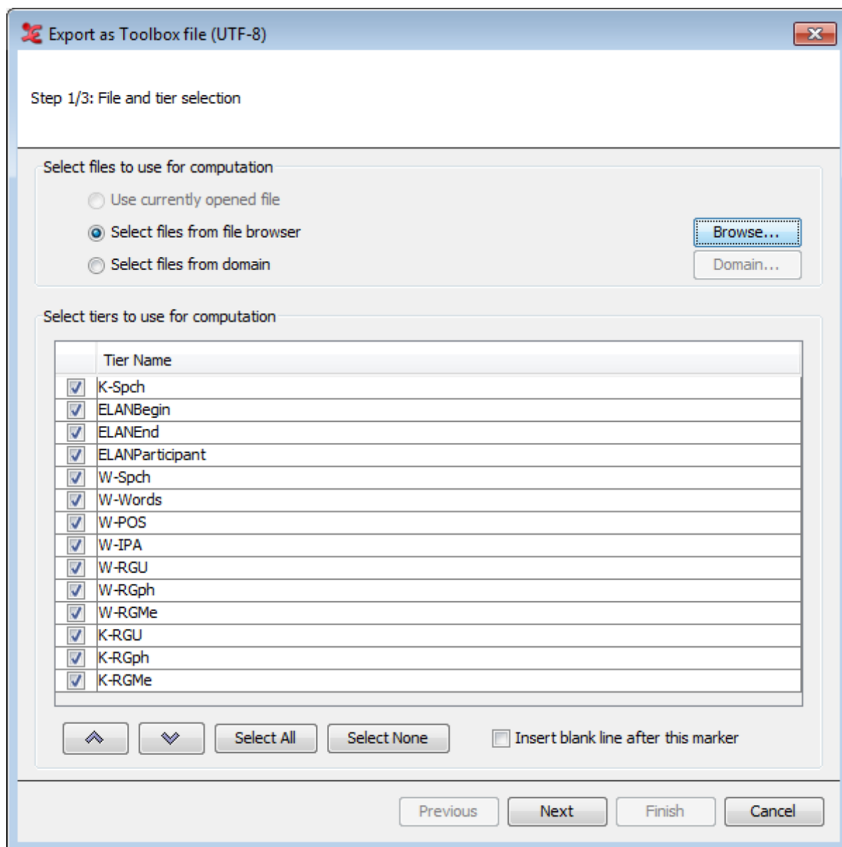
Figure 1.153. Export as Toolbox file step 1
