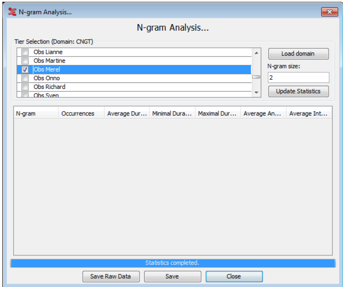
Figure 1.144. N-Gram Analysis dialog 2
