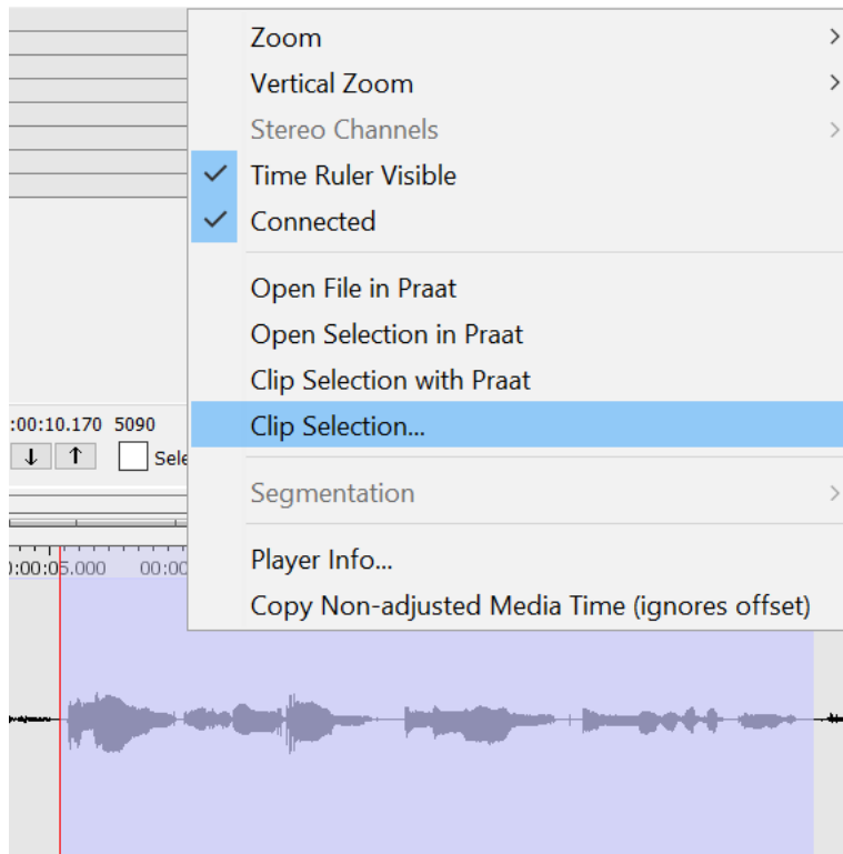
Figure 1.75. Waveform context menu
