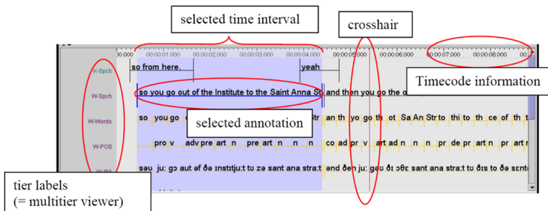
Figure 1.85. The timeline viewer
